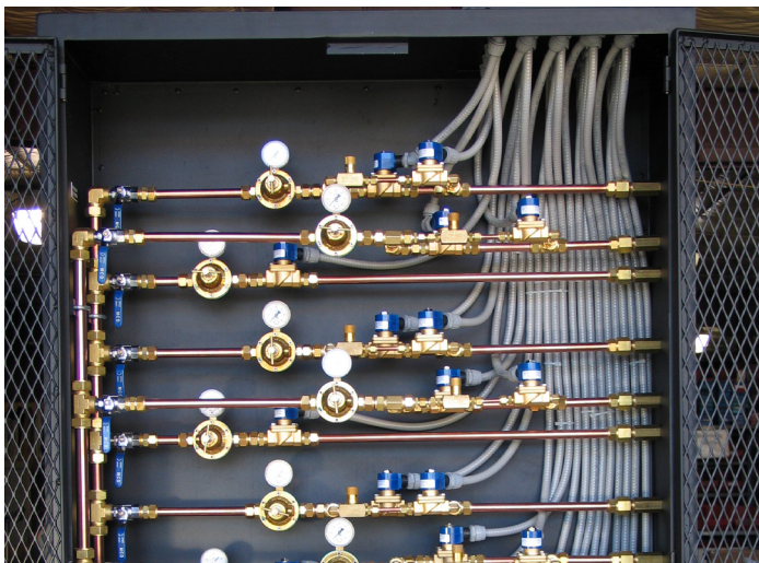
Gas Mizer Manifolds
