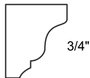
5/8" 3/4" Neck Mould
