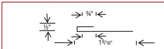
1/2" J-Channel (Aluminum)
