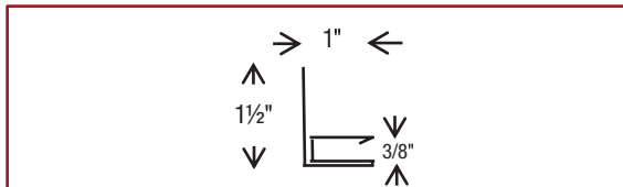
3/8" F-Trim (Aluminum)
