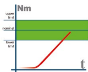
Torque/Time
