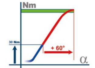
Tightening with torque and additional angle rotation (torque + angle)
