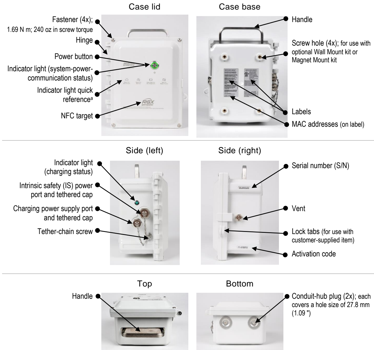
Figure 1.2.A Hardware overview (exterior)
